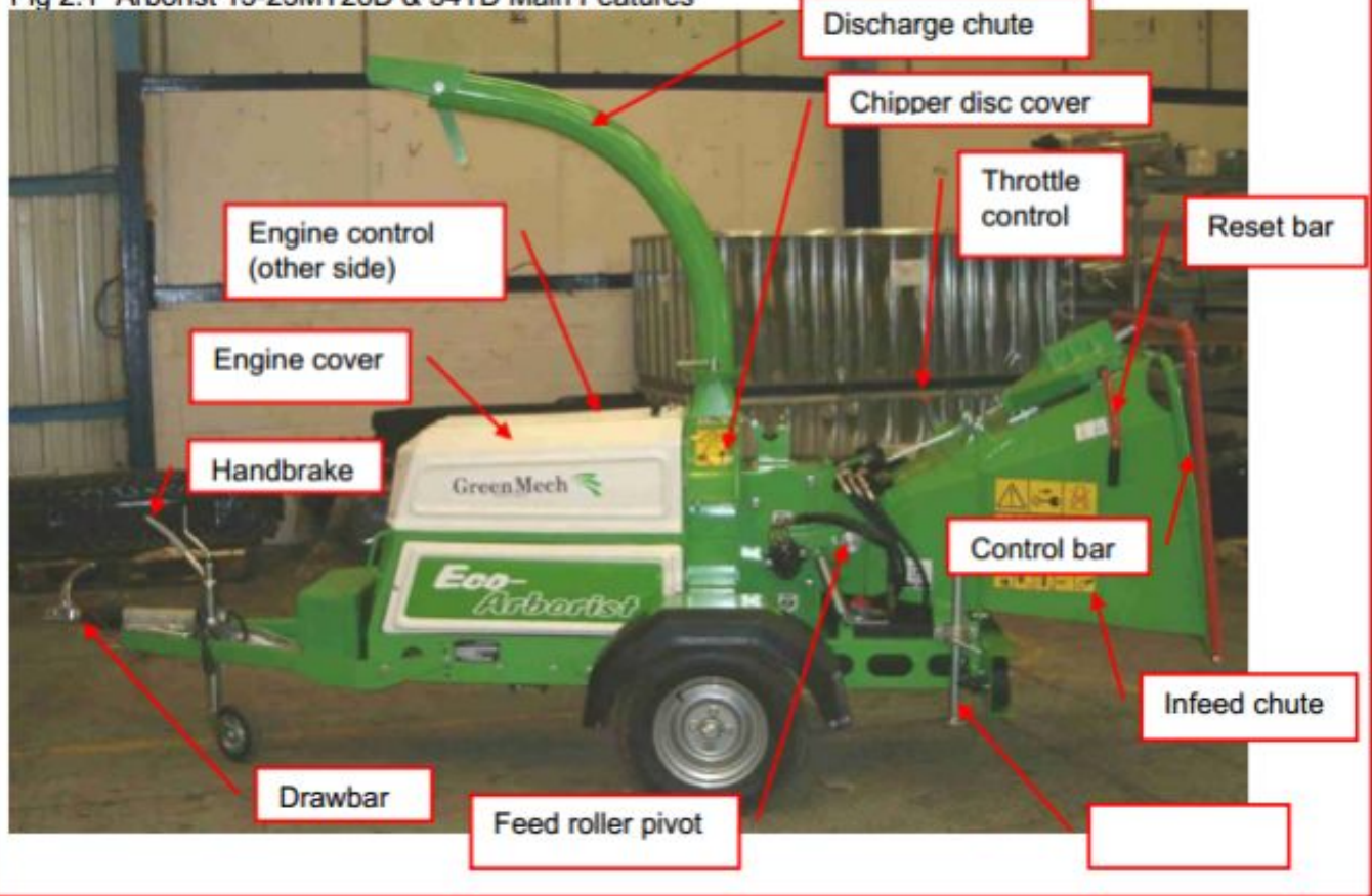
Fig 2.1 Arborist 15-23MT26D & 34TD Main Features
